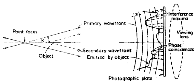
Fig. 1. INTERFERENCE BETWEEN HOMOCENTRIC ILLUMINATING WAVE AND THE SECONDARY WAVE EMITTED BY A SMALL OBJECT
